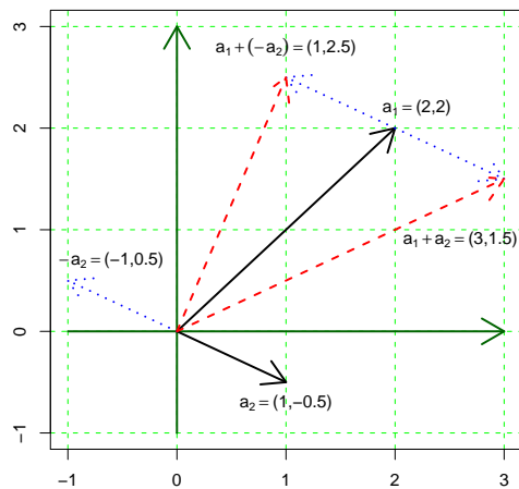
Figure 4: Addition of vectors and multiplication by a number
