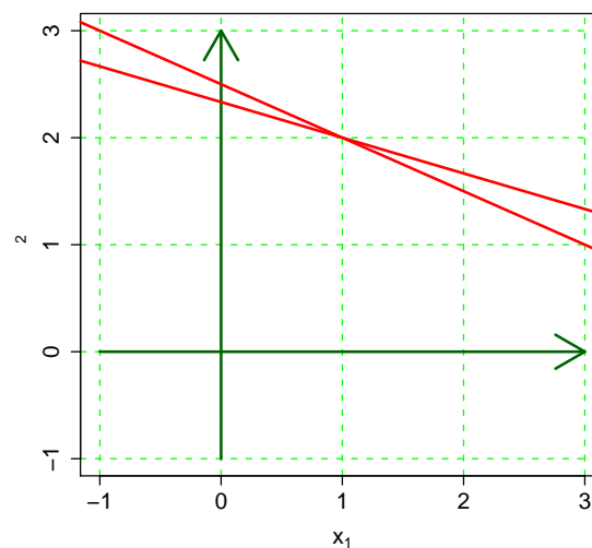
Figure 5: Solving two equations with two unknowns.
