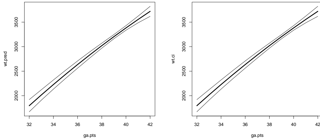
Figure 7: Prediction of the gestational age-specific birth weight. Left panel computed “by hand”, right panel using ci.lin .
