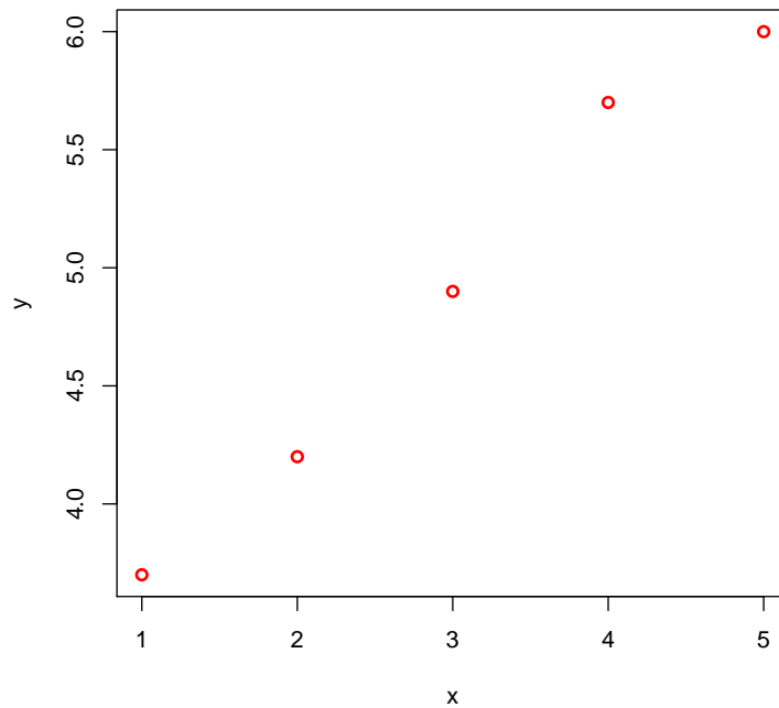
Figure 6: Regression
