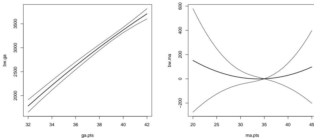
Figure 8: Prediction of the gestational age-specific birth weight for maternal age 35 (left) and the effect of maternal age on birth weight, relative to age 35.
