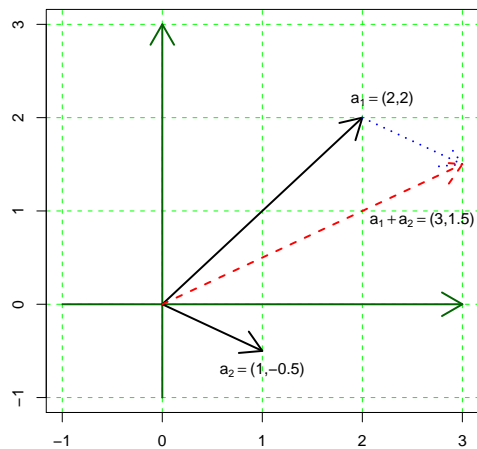
Figure 3: Addition of vectors
